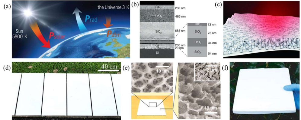
Figure 1. Principle of radiative cooling and high-performance radiative cooling materials. (a) Principle diagram of radiative cooling [2], where P_{rad} represents thermal radiation, P_{atm} represents absorbed atmospheric radiation, and P_{solar} represents absorbed solar radiation. (b) Multilayer film photonic crystal alternately composed of SiO 2 and HfO 2 [8]. (c) Metamaterial film formed by SiO 2 particles incorporated into polymethylpentene matrix [9]. (d) Ultra-white coating formed by mixing TiO 2 and fluoropolymer [10]. (e) Hierarchically porous membrane prepared by phase inversion method [11]. (f) Delignified pressed ultra-white wood [12].
